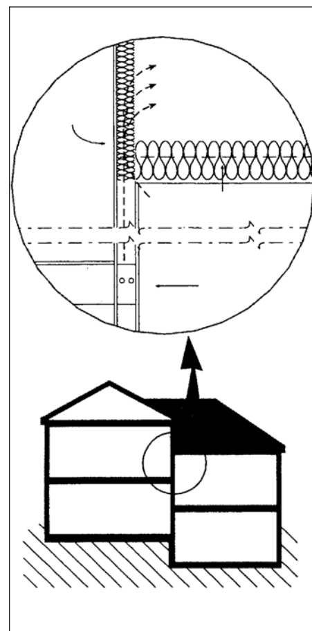
Figure 2 Leakage areas on split level houses
